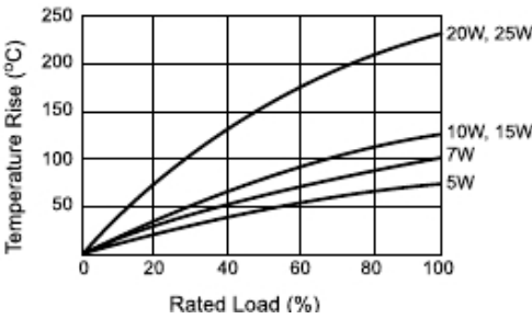
Heat Rise Chart (PRS)
