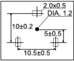
PRS 7W, 10W, 15W
